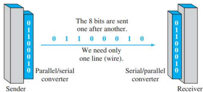
Figure 4.33 Serial transmission
