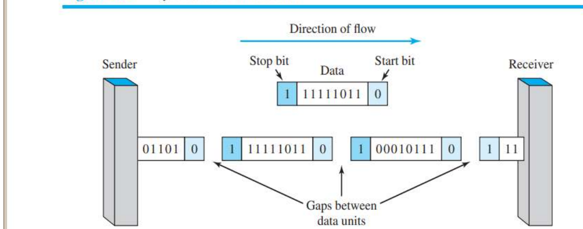
Figure 4.34 Asynchronous transmission
